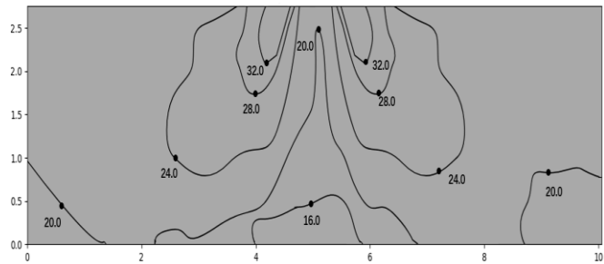
Figure 9.40: MIH180Q4HN18 heating at 300s
