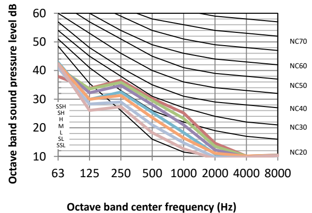
Figure 8.5: MIH56Q4HN18 octave band levels
