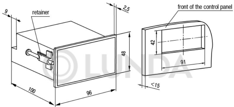
Figure 4.7 – Dimensions of \sqcup 2 housing
