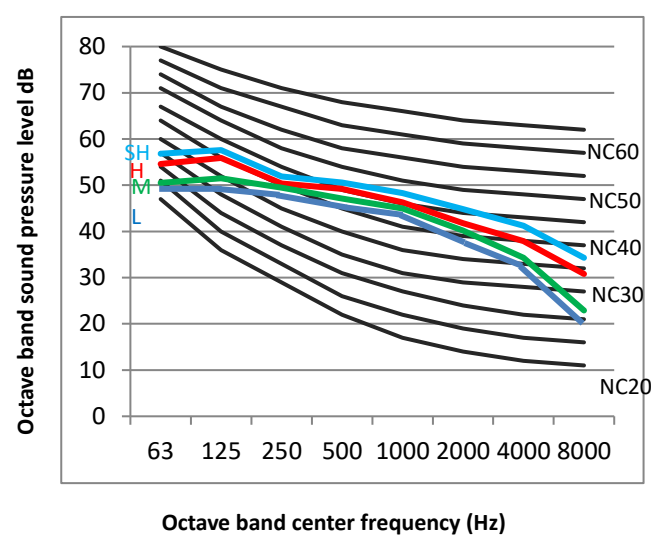
Figure 9.5: MDV-D160T1/N1-B(B) octave band levels
