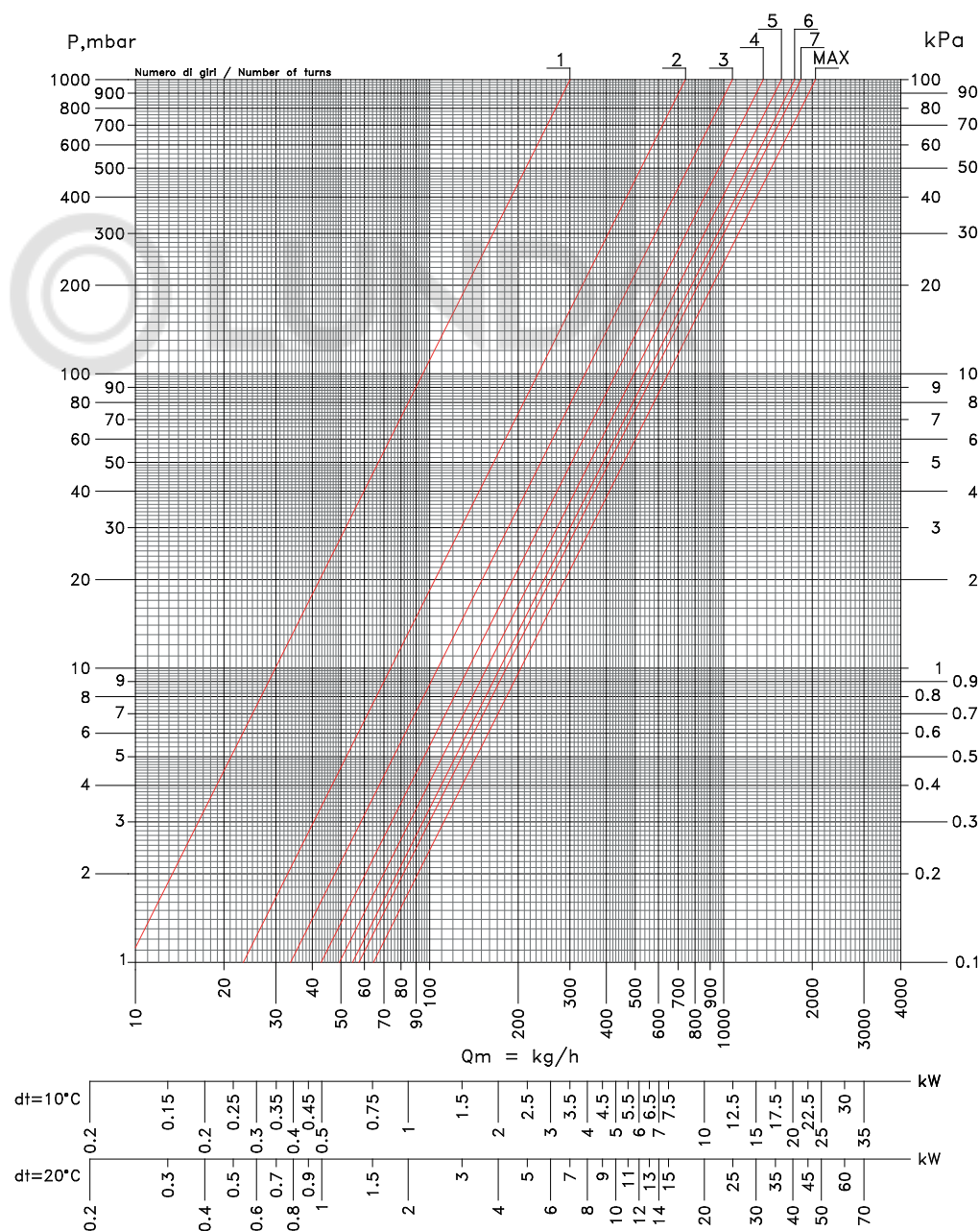
TWIN THERMO PRESET BITUBE ANGLE DN 15 1/2"
