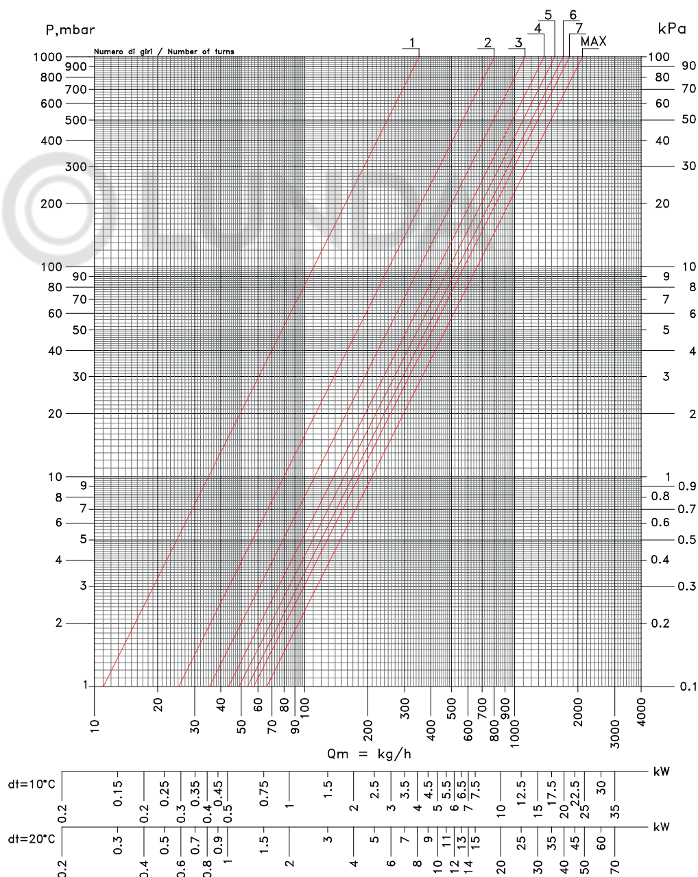
TWIN THERMO PRESET BITUBE STRAIGHT DN 15 1/2"
