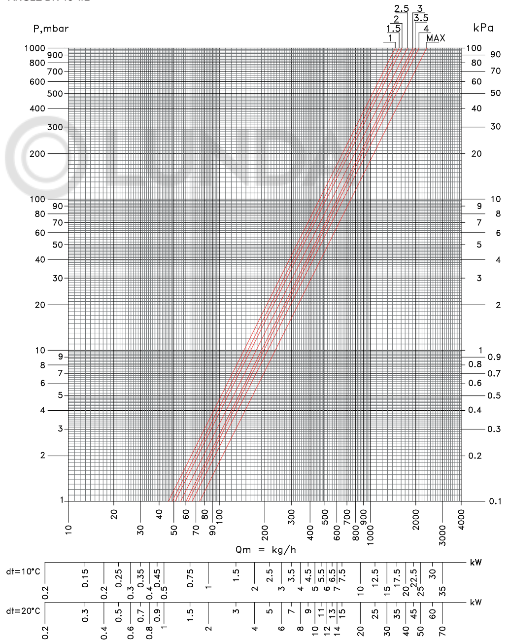
TWIN LOCKSHIELD MONOTUBE ANGLE DN 15 1/2"
