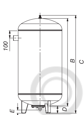
Flexcon RM 110–300
