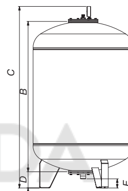
Flexcon RM 425–1000
