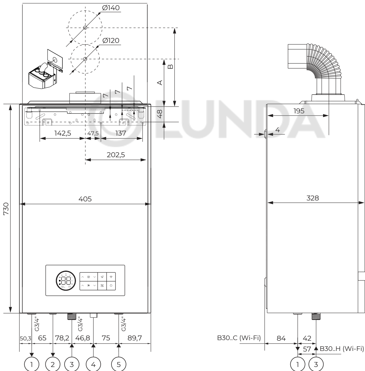
Рис. 43. B30 28 C/H (Wi-Fi), B30 32 C/H (Wi-Fi), B30 36 C/H (Wi-Fi).
