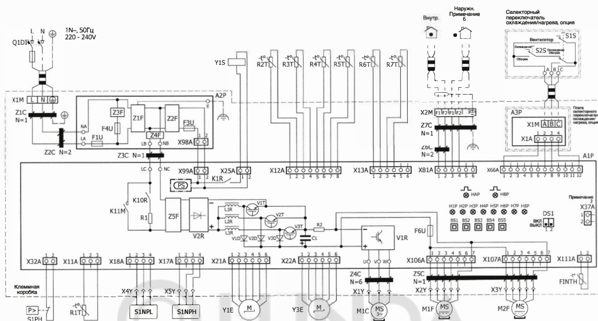
RXYSQ-T8V
