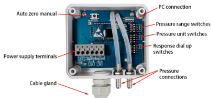
Figure 1 LFM11X-XAX Internal Circuit
