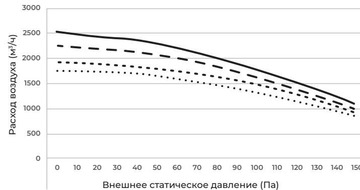
LAC-DR165HP.D01/S
