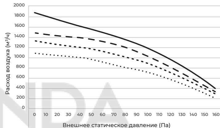
LAC-DR140HP.D01/S
